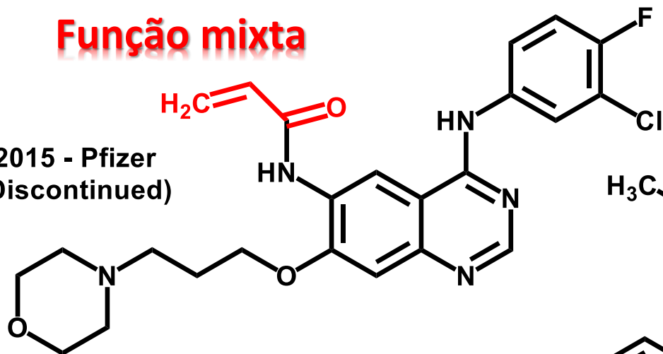
Canertinibe
