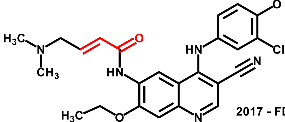
Neratinibe
